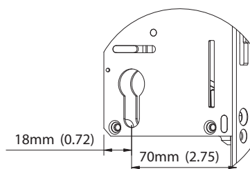
Gear - 70mm Backset
