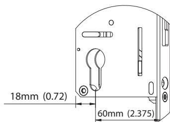
Gear - 60mm Backset
